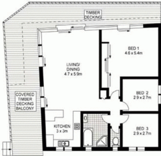
UPPER LEVEL
