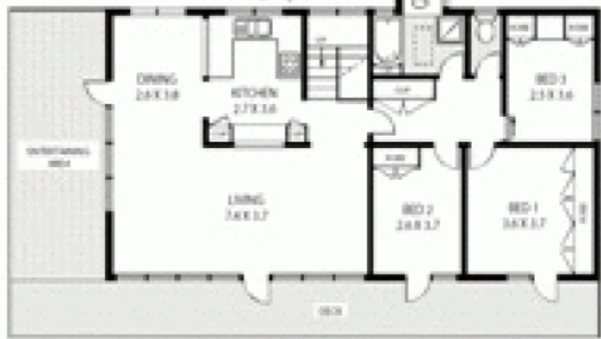
UPPER GROUND FLOOR
