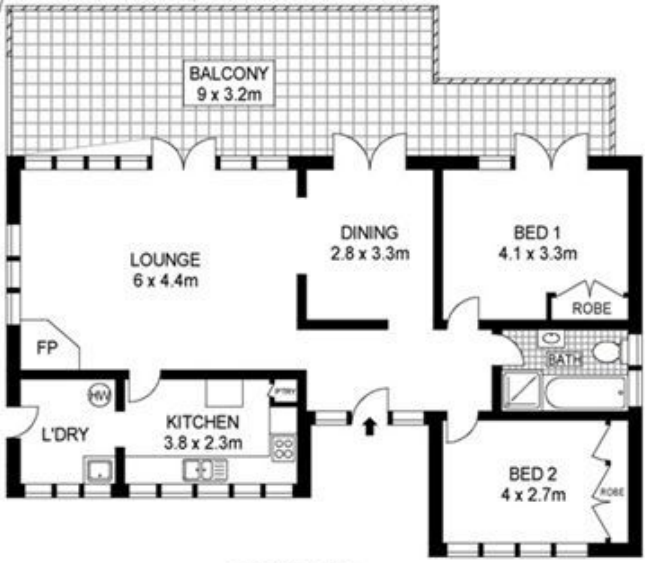
GROUND LEVEL
